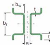
I cartola (FF)
