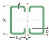
2 U (FF) enrijecidos
