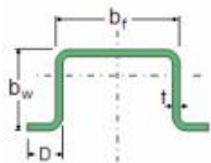
Cartola (FF)
